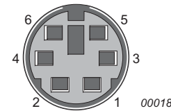
Figure 3: Line identities of the Alarm / RS 232 socket, viewed externally (i.e. also from the solder bucket side of the plug)
