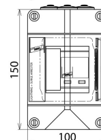
Dimension drawing DSP 12 SH 240 TT
