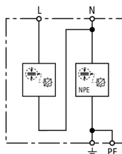
Basic circuit diagram DSP 12 SH 240 TT
