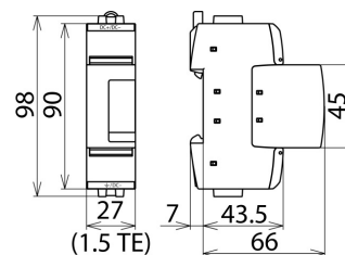
Dimension drawing DG SE DC 242
