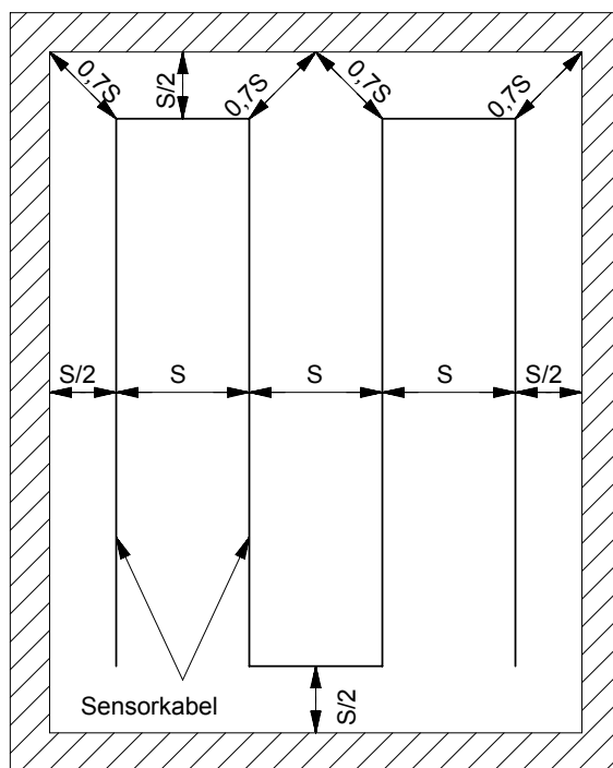
Fig. 3.7: Installation of the "Alarmline" sensor cable for room protection
