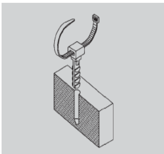
Fig. 3.10: Assembly base for cable fixings (FTH 20)
