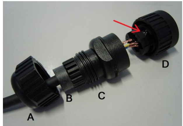
DNA212 comes with MG2257 free connector. Pass the cable as in the picture above, select the rubber ring B ( \varnothing 6 or 9 according to the cable dimension). Then fix the wires to the connector as in the drawing on the left. Read also DISACC 5635 drawing.
