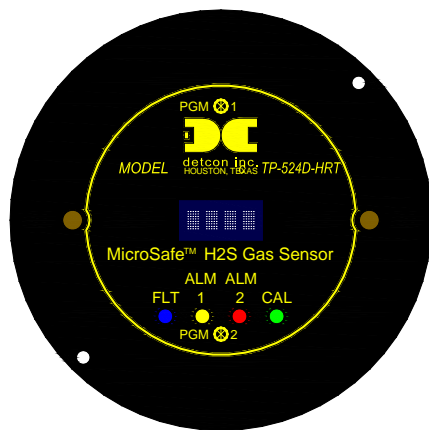
Figure 3 Transmitter Module
