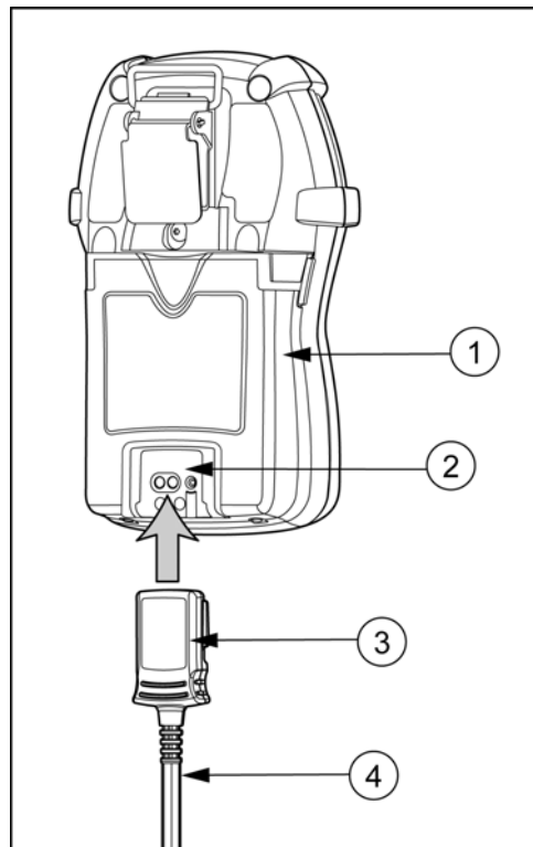
Figure 16. Connecting the Charger Adapter
